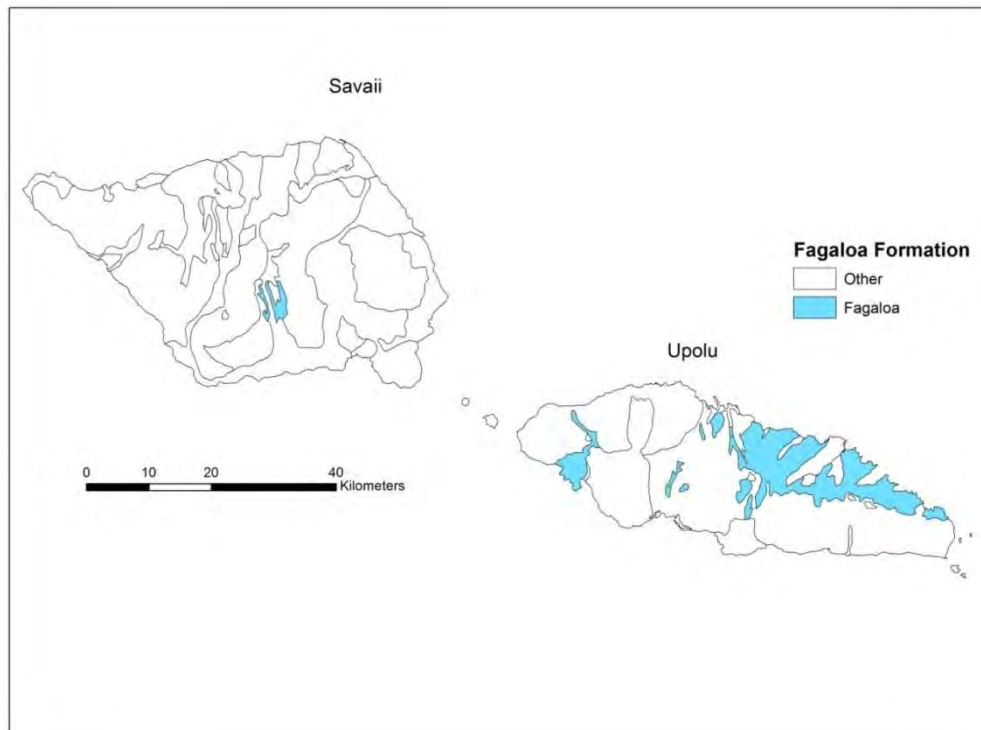
Figure 5. Fagaloa Formation.
